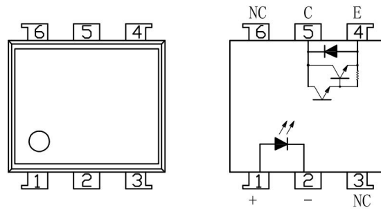
图 2 电原理图 Figure 2-Schematic
