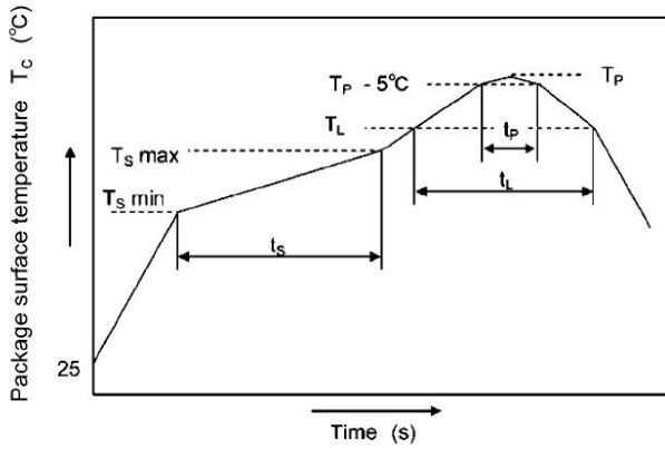
Figure 7-Recommended reflow soldering profile
