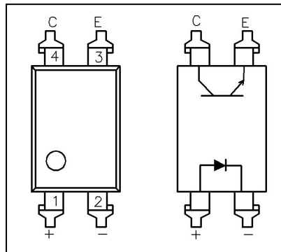
图3 电原理图 Figure 3-Schematic
