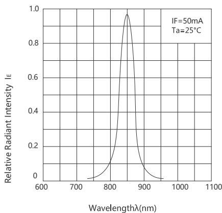
Fig.7 Relative Radiant Intensity vs. Wavelength
