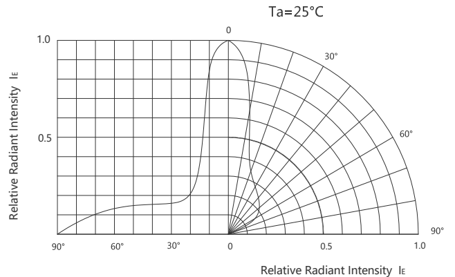
Fig.8 Relative Radiant Intensity vs. Angular Displacement
